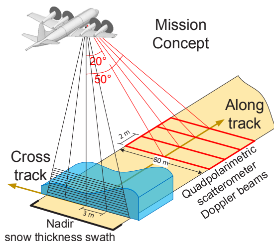
Figure 36. Mission concept for multichannel snow radar instrument flights. Figure credit: John Paden
